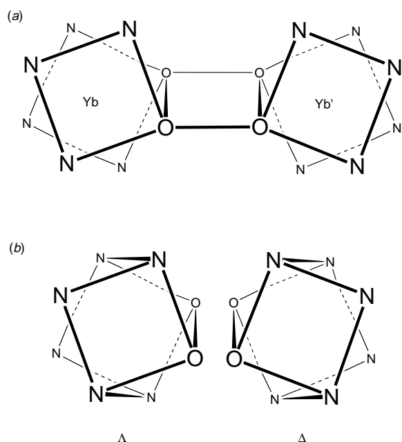
Fig. 5 (a) Schematic drawing of Ni(tdo)Yb 2 and (b) proposed definition of the absolute configuration (Λ and Δ) of the square antiprism
